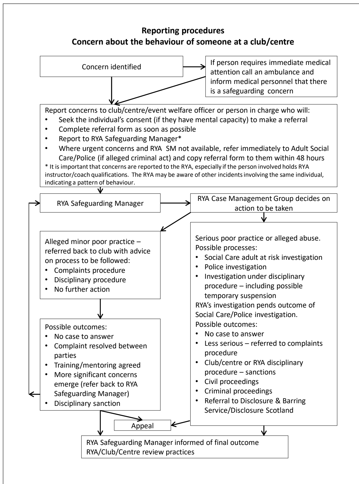
Flowchart 2
