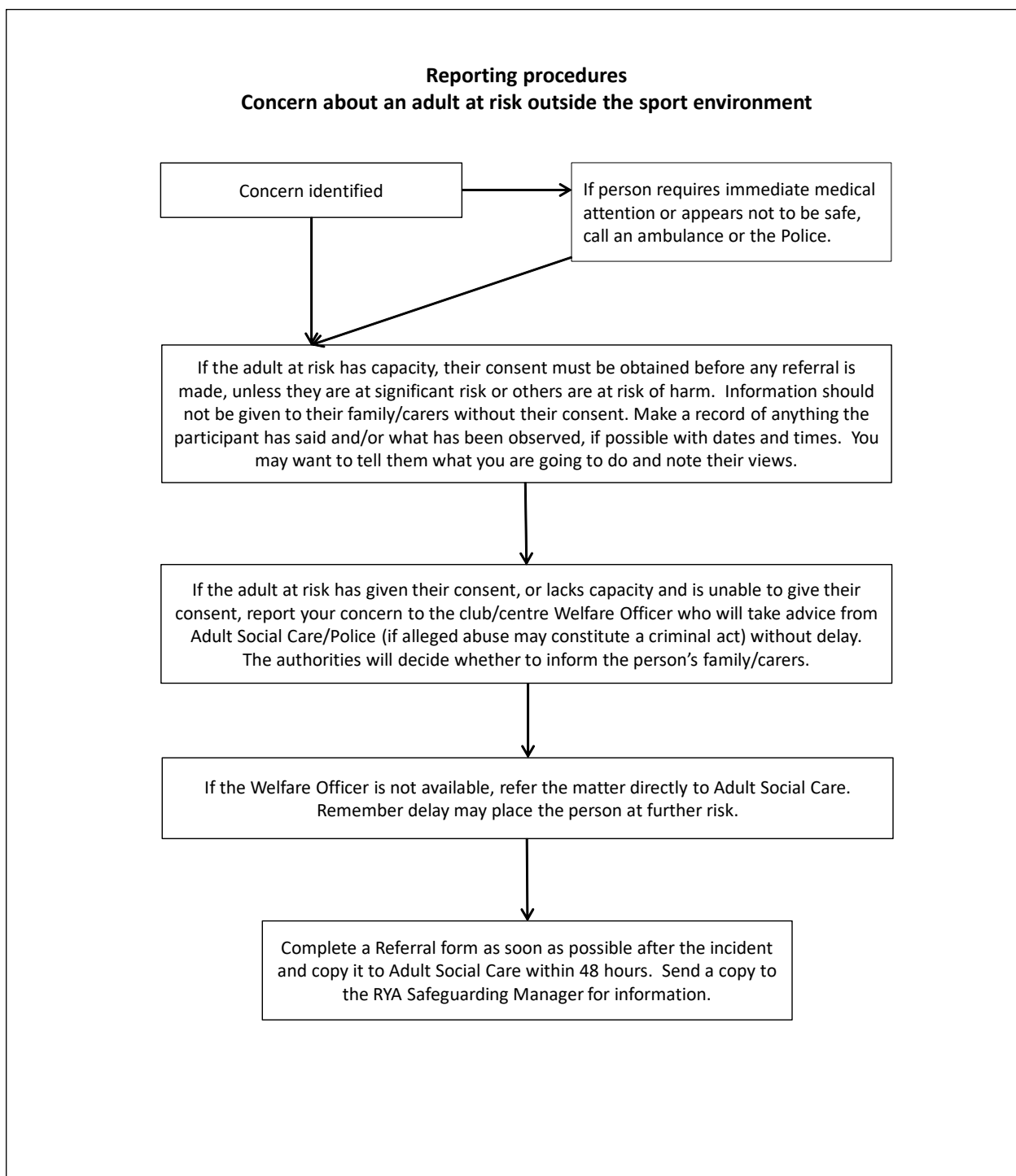
Flowchart 1
